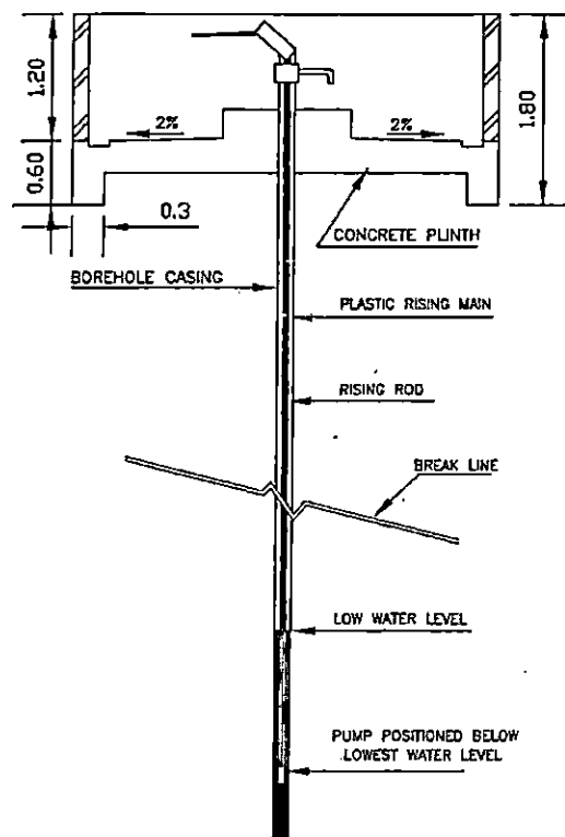
CROSS SECTION BOREHOLE MENVA
