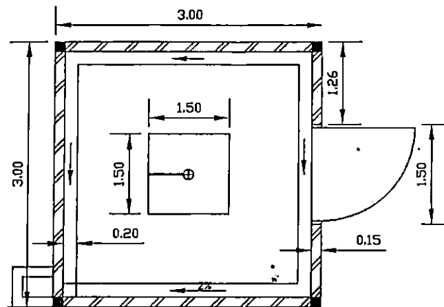
PLAN OF COLLECTION POINT
